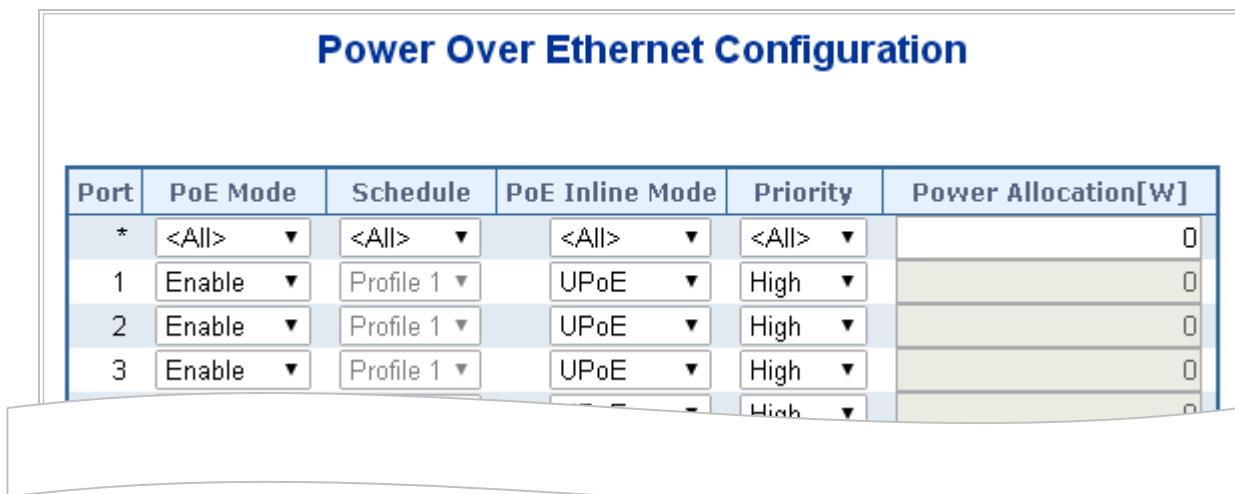
Figure 4-7-1-3: Power over Ethernet Configuration Screenshot
