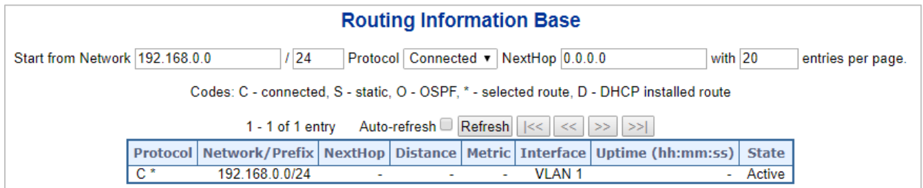
Figure 4-2-3: IP Status Page Screenshot
