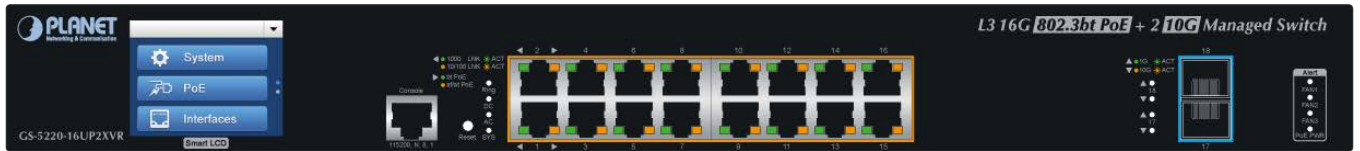
Figure 2-1-6: Front Panel of GS-5220-16UP2XVR
