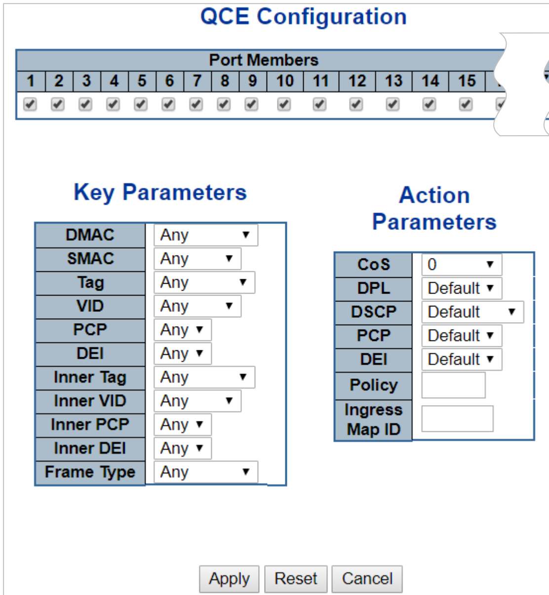
Figure 4-5-5-2: QCE Configuration Page Screenshot
