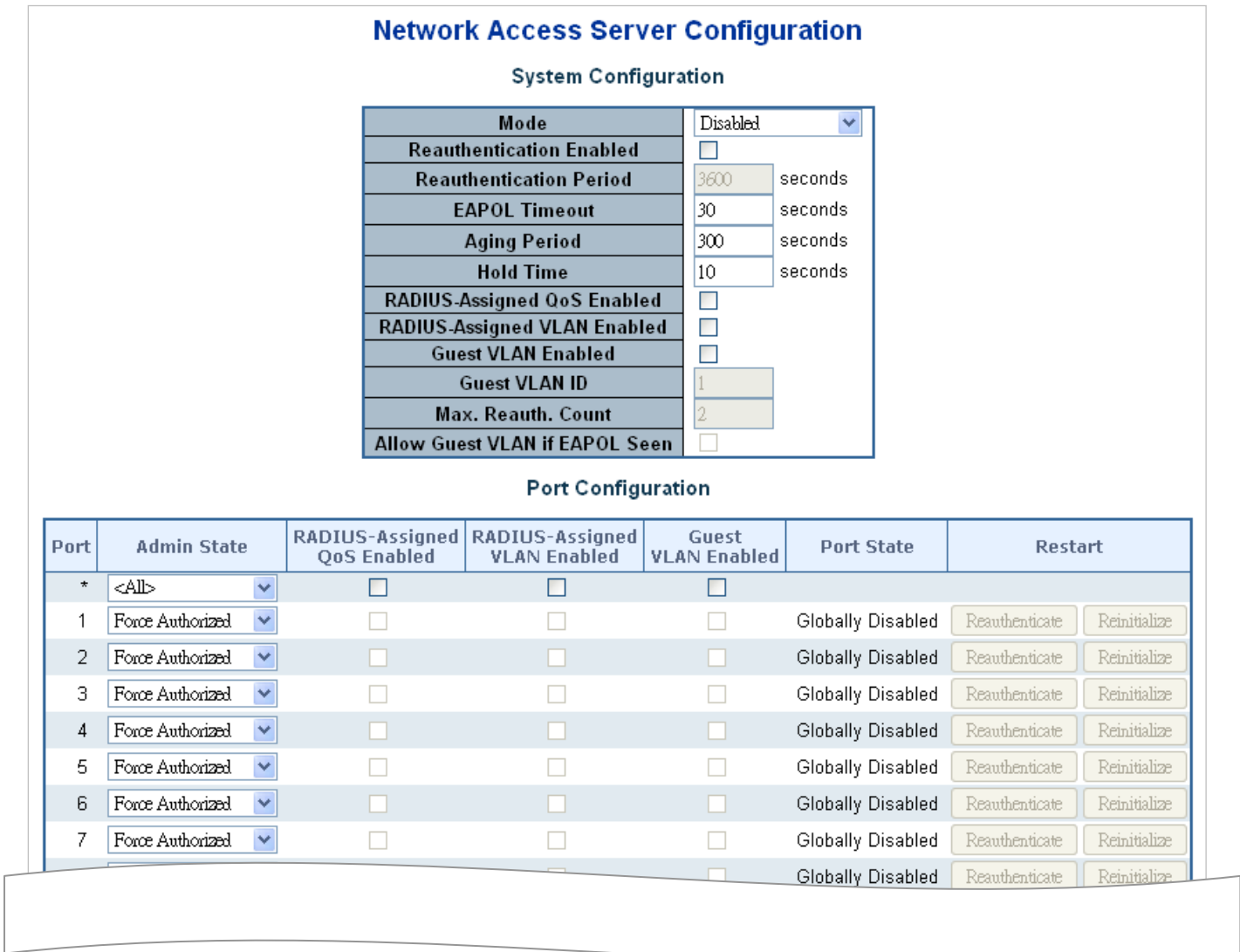
Figure 4-6-3-1: Network Access Server Configuration Page Screenshot
