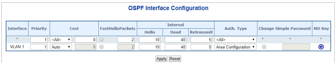
Figure 4-4-4-7: Interface Configuration Page Screenshot
