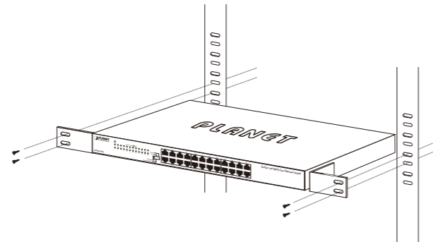
Figure 5: Mounting the Fast Ethernet Switch in a Rack
