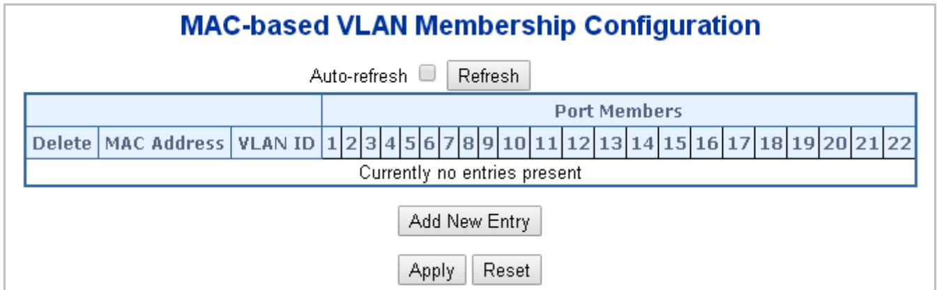
Figure 4-6-18: MAC-based VLAN Membership Configuration Page Screenshot
