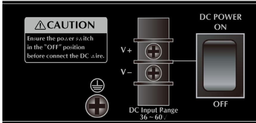
Figure 2-1-35 Rear Panel of GS-5220 Redundant Power Models
