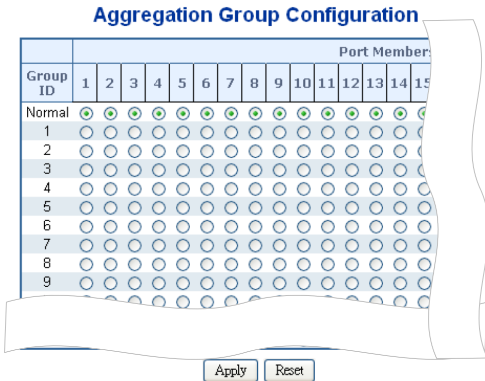
Figure 4-5-3: Aggregation Group Configuration Page Screenshot
