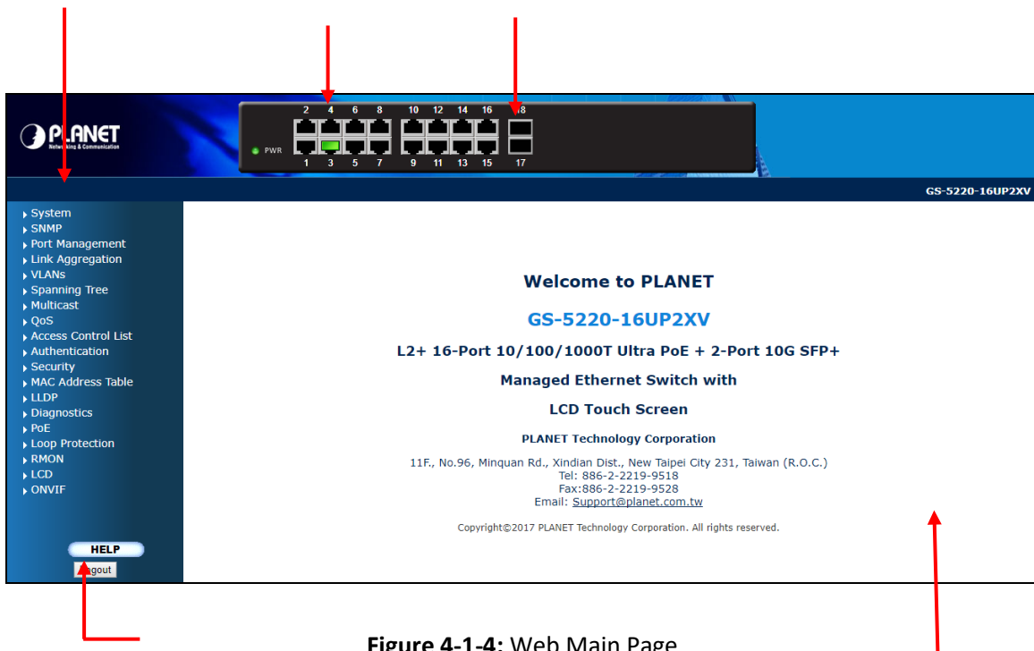
Figure 4-1-4: Web Main Page
