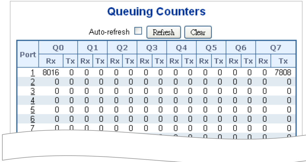
Figure 4-9-17: Queuing Counters Page Screenshot
