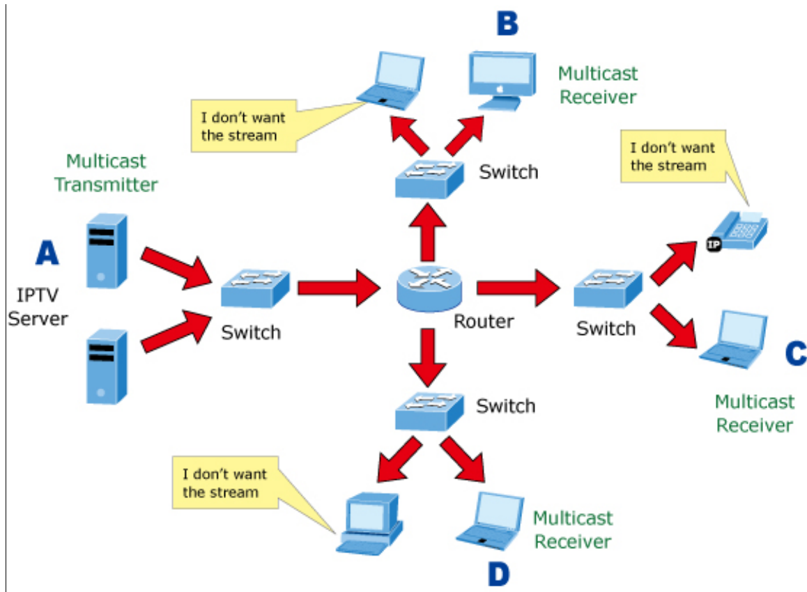
Figure 4-3-5-2: Multicast Flooding
