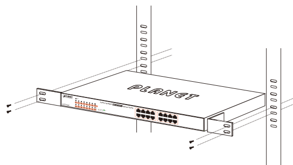
Figure 5-3: Mounting the Switch in a Rack
